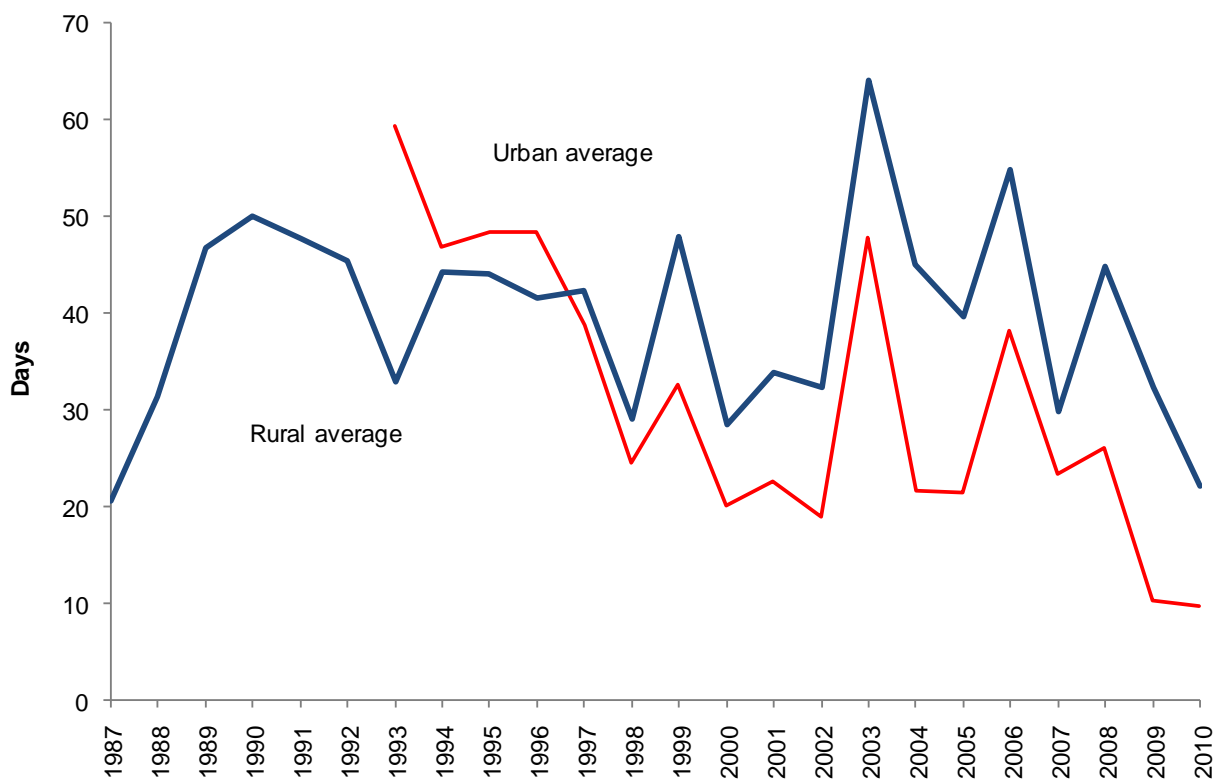
Figure 2: Number of days when air pollution is moderate or higher, 1987-2010 (provisional), UK
