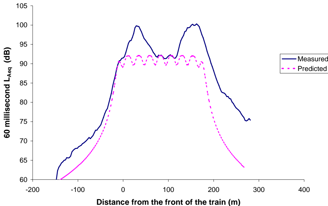
Figure 6 Typical Measured and Predicted Time History for two Class 220 Voyagers coupled together
