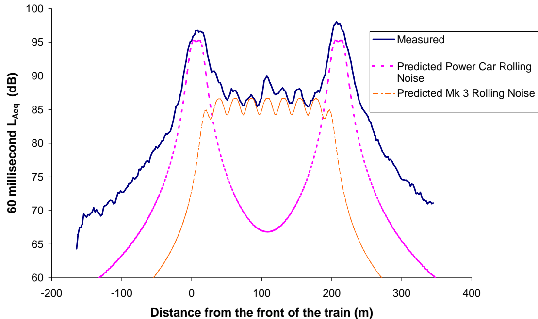
Figure 4 Predicted and Measured Time History of a Train Pass-by with the Predicted Levels for the Power Cars and Mk III coaches separated
