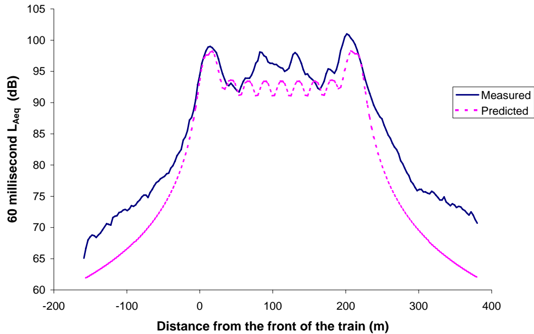
Figure 5 The Measured and Predicted Rolling Noise Time History for a Second HST
