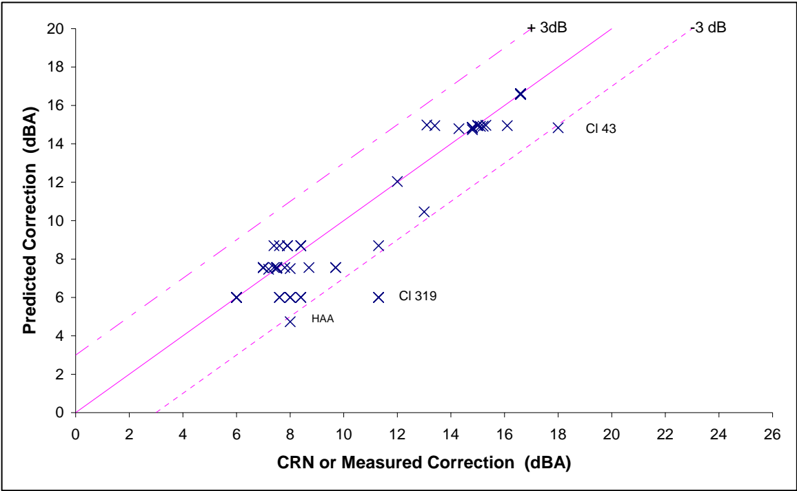
Figure 1 CRN corrections predicted using the AEA Technology methodology vs values either in the CRN 1995 document or obtained from measurement
