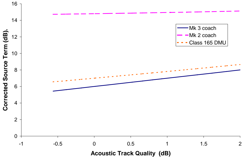
Figure 7 Effect of Acoustic Track Quality on the Corrected Source Terms
