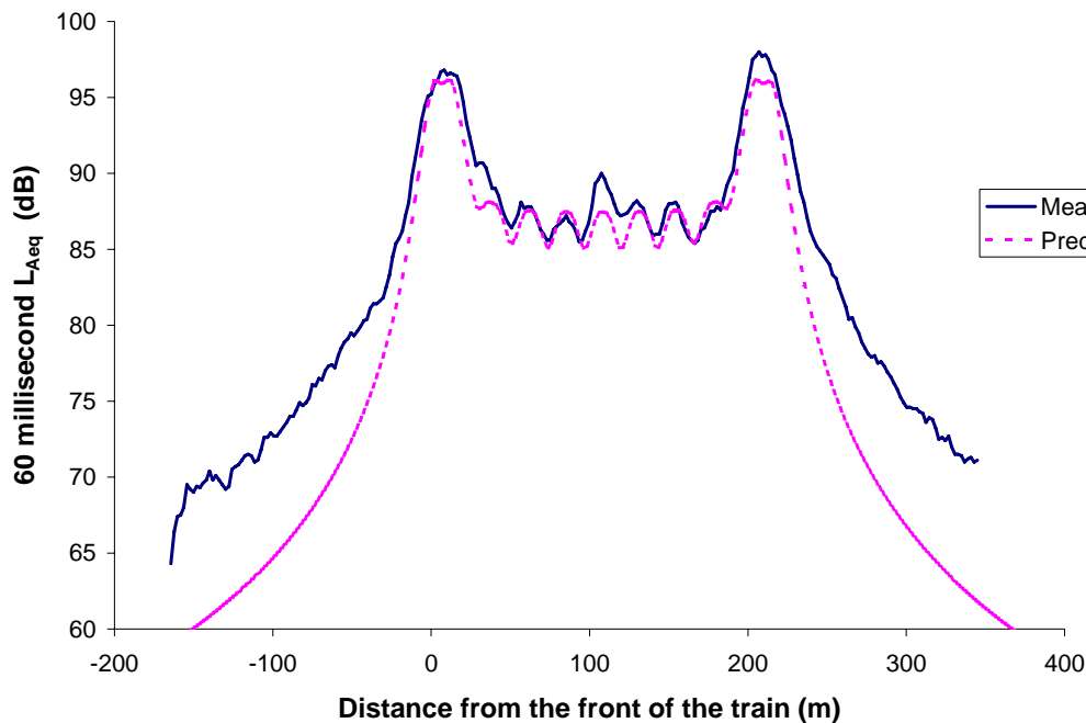
Figure 2 Typical Measured and Predicted Time History of a Train Pass-by
