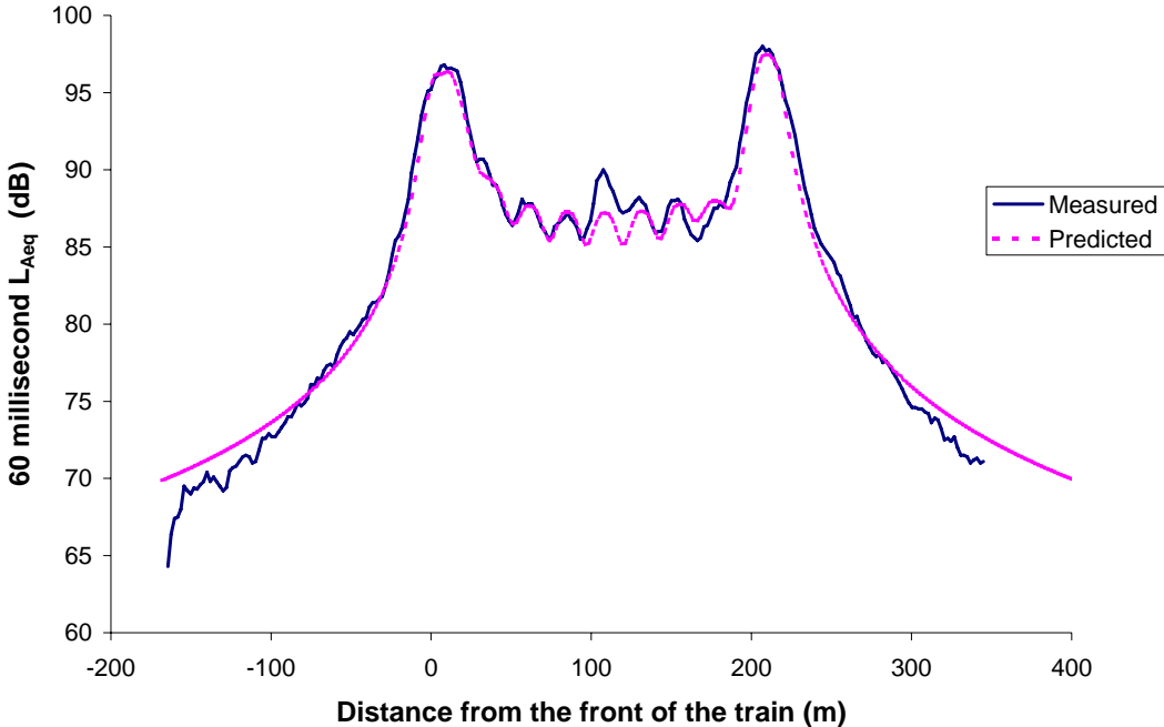
Figure 3 Typical Measured and Predicted Time History of a Train Pass-by with the Prediction including Engine Noise
